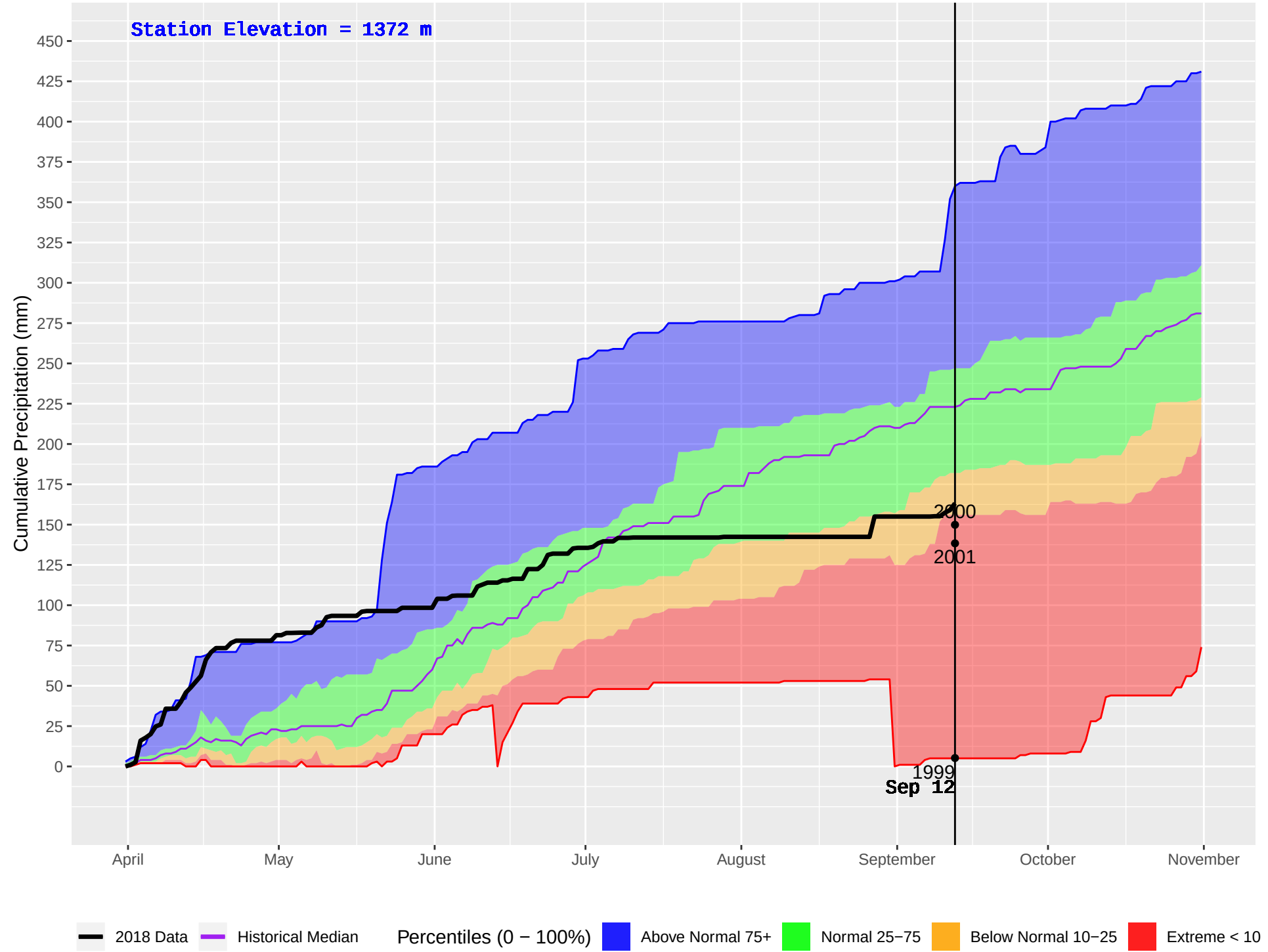
CHERRY LAKE (791) : Historical (1989–2016) and Current (2018) Daily Cumulative Precipitation
