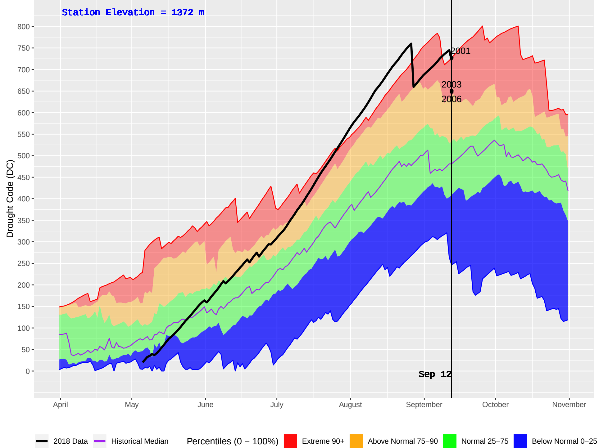
CHERRY LAKE (791) : Historical (1989–2016) and Current (2018) Daily Drought Code (DC)
