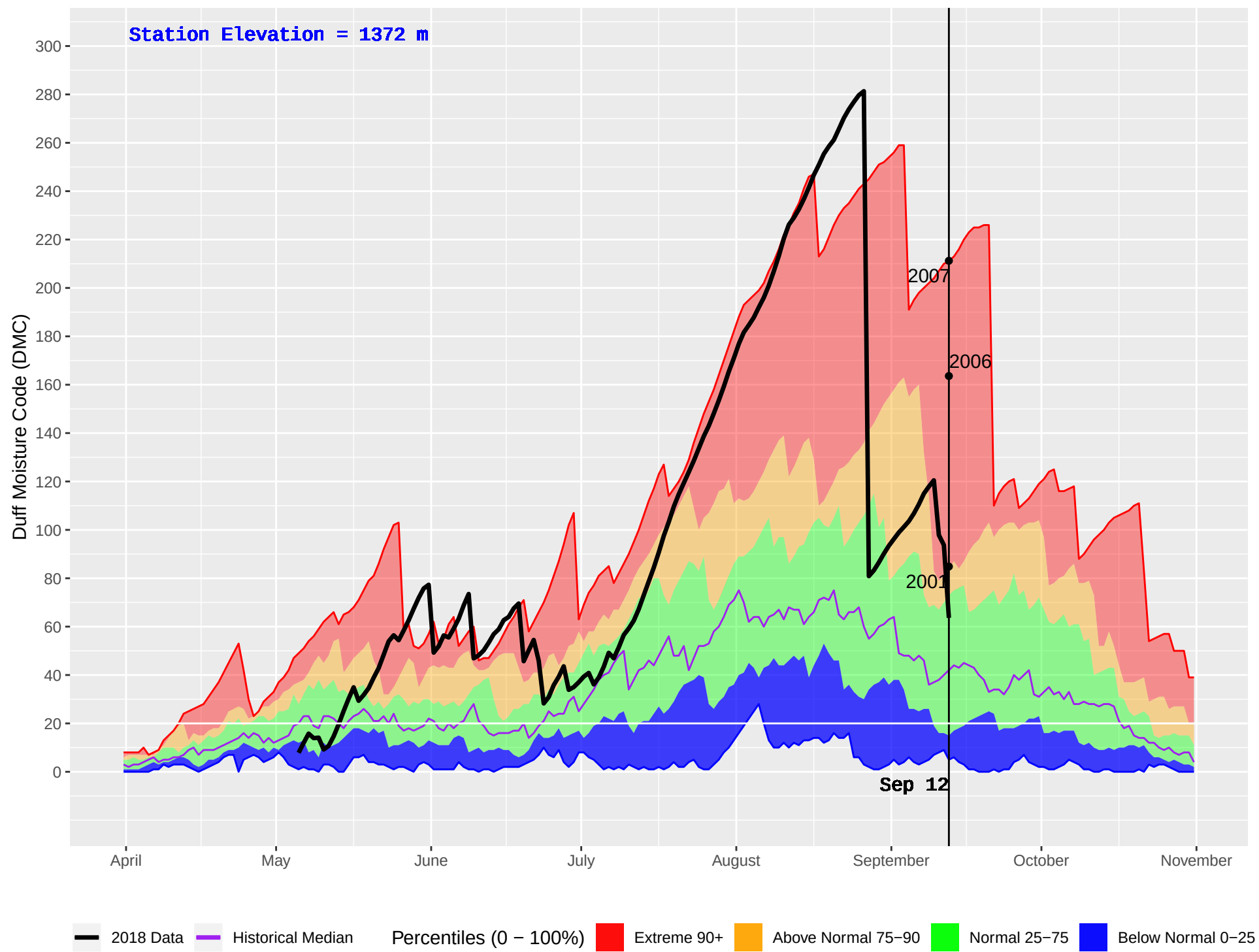
CHERRY LAKE (791) : Historical (1989–2016) and Current (2018) Daily Duff Moisture Code (DMC)
