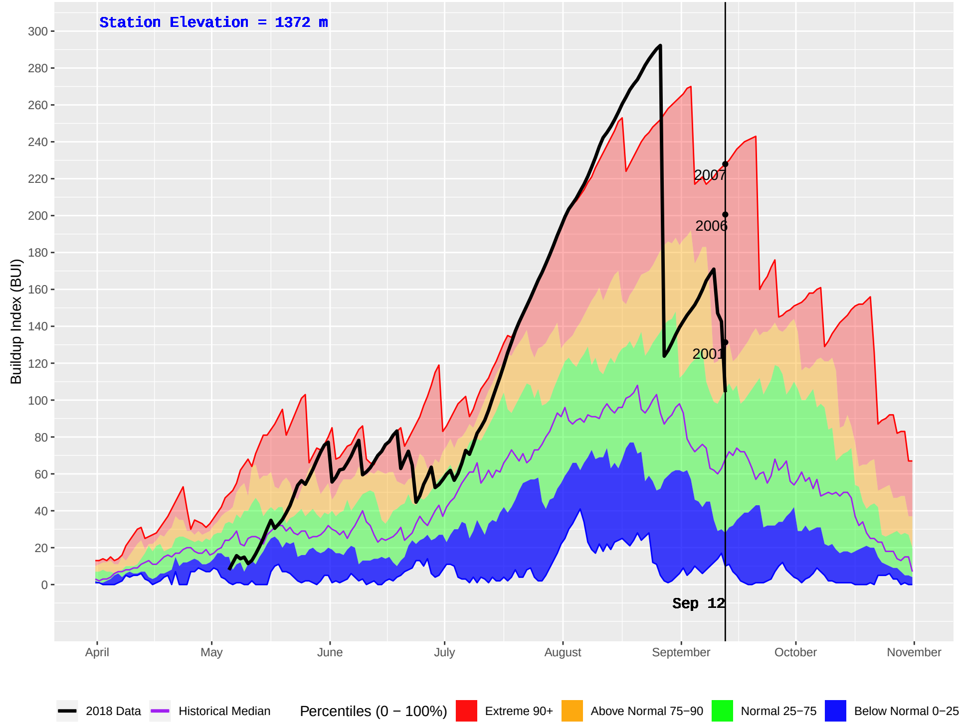
CHERRY LAKE (791) : Historical (1989–2016) and Current (2018) Daily Buildup Index (BUI)
