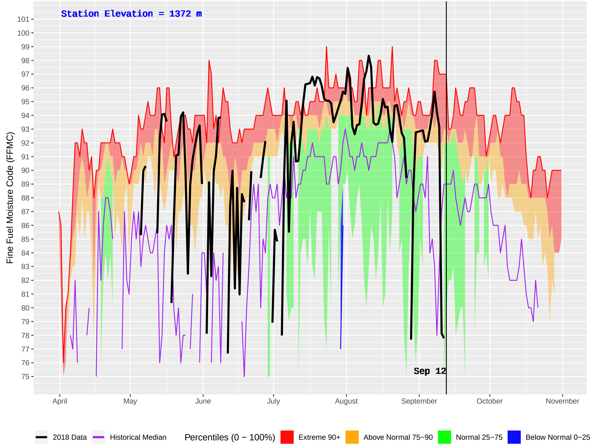
CHERRY LAKE (791) : Historical (1989–2016) and Current (2018) Daily Fine Fuel Moisture Code (FFMC)
