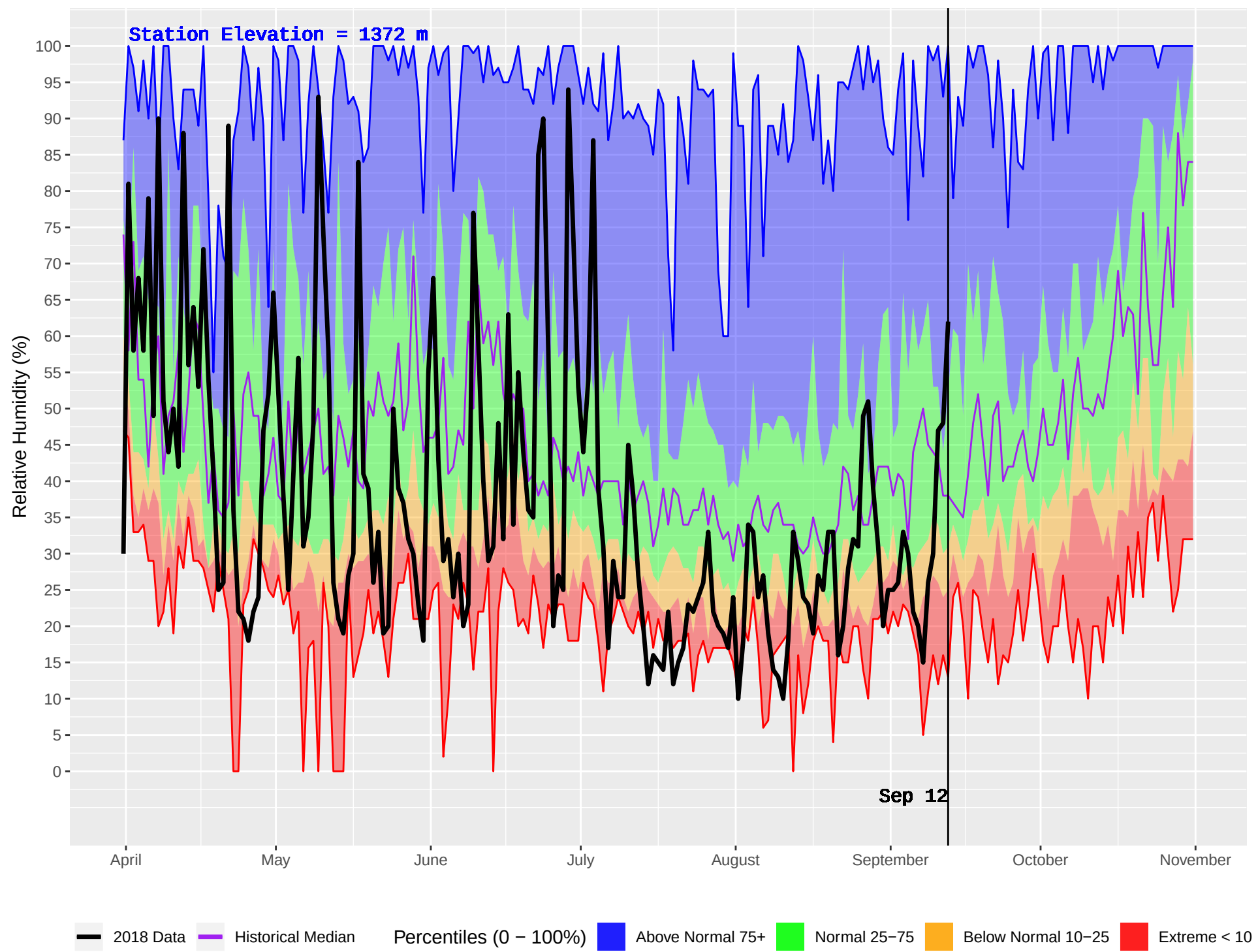
CHERRY LAKE (791) : Historical (1989–2016) and Current (2018) Daily Relative Humidity
